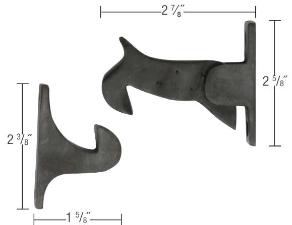
1083 Door Holder Shown in dark bronze patina
