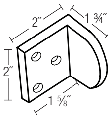
3550.1 3/4 Standard Gate Stop
