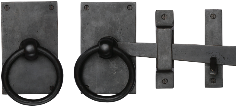
3510 Ring Turn Drop Bar Plate size: 4 1/2" x 2 3/4" Ring Dia: 3 1/8" Arm Length: 6 1/2" Handing required. Right hand pictured Must be used in conjunction with a gate stop.
